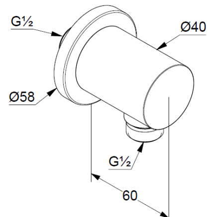
Dimensional drawing
