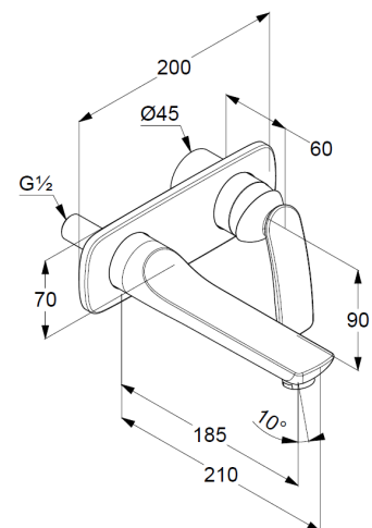
Dimensional drawing
