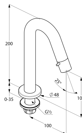
Dimensional drawing
