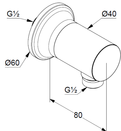
Dimensional drawing
