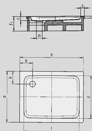
Illustration shows Model 546-2
