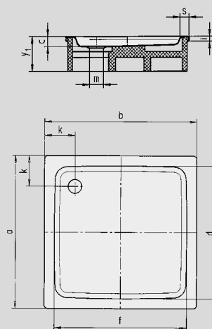
Illustration shows Model 545-2
