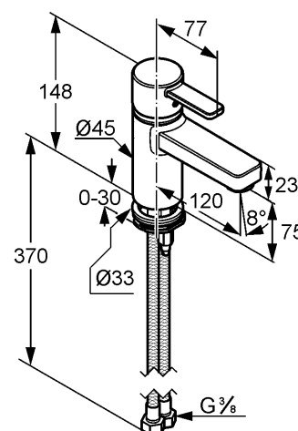
Dimensional drawing
